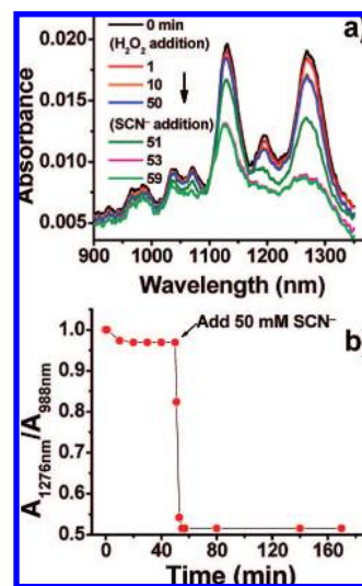
Figure 2. (a) Time-dependent NIR absorption spectra and (b) time-dependent, normalized A_{1276\text{nm}}/A_{988\text{nm}} of a 100 ppm H 2 O 2 -reacting ssDNA-SWNT sample in 2-(4-morpholino)ethanesulfonic acid (MES) buffer before and after addition of 50 mM SCN − .
