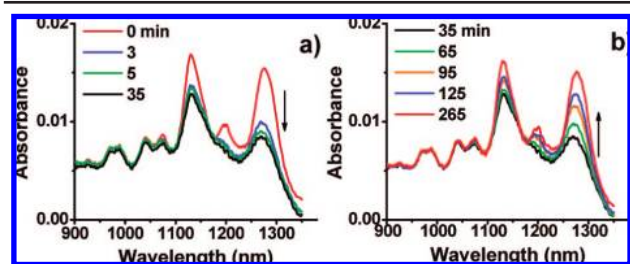
Figure 3. NIR absorption spectra of an ssDNA-SWNT sample in MES buffer containing 1 M \text{SCN}^- change as a function of time after addition of 100 ppm \text{H}_2\text{O}_2 : (a) suppression and (b) recovery in spectral intensity.
